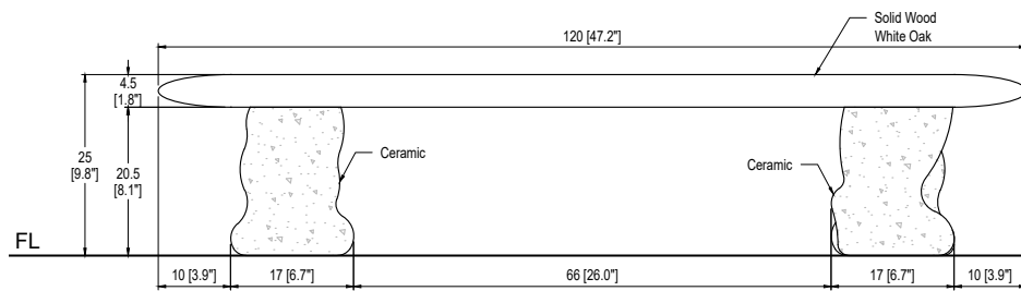
FRONT VIEW Scale 1:8
